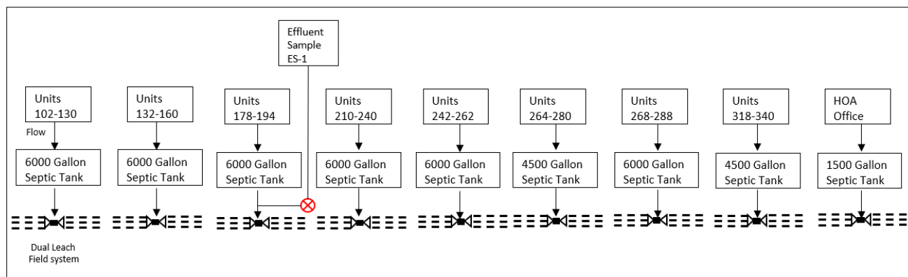
Figure 1. Process Flow Diagram with Sampling Locations
