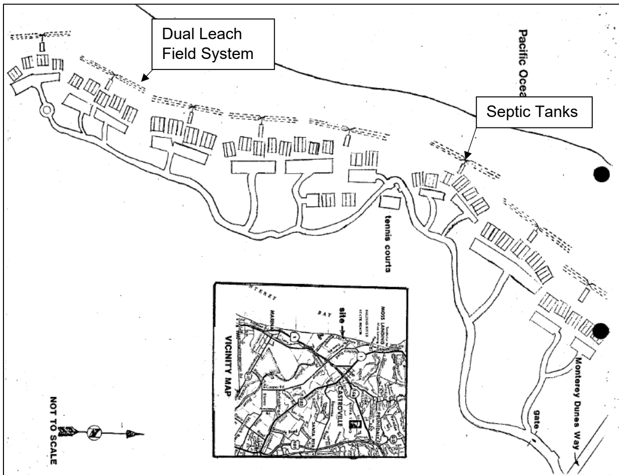
Figure 3. Dispersal System Layout
